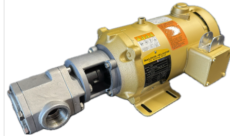
Stainless Steel 25GPM Oil Transfer Pump
