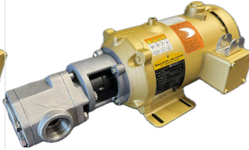
Stainless Steel 12GPM Oil Transfer Pump
