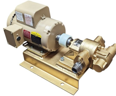
Industrial 10GPM with Bypass 480V
