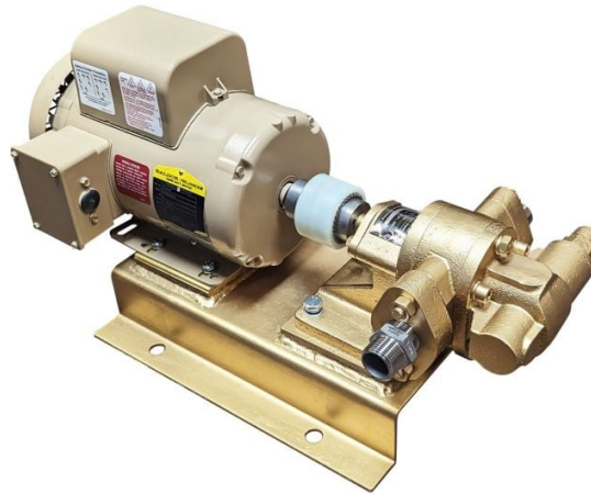
Industrial Oil Transfer Pump - 60GPM
