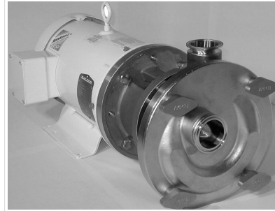
Low Vibration Sanitary Pump 100GPM
